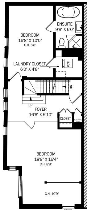
SECOND FLOOR - 801 SQUARE FEET
